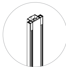
Wall Start Double Glass (MFWSDG) • Adjustable wall start for monolithic double glass fascias against drywall
