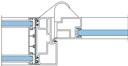
Wall Door Start Double Glass (MFWWDSG)
