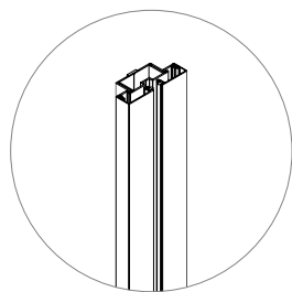
Wall Start Single Centered Glass (MFWSSC) • Adjustable wall start for monolithic single centered glass fascias against drywall
