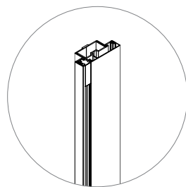
Wall Start Single Offset Glass (MFWSSO) • Adjustable wall start for monolithic single offset glass fascias against drywall
