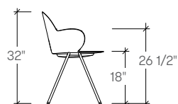
Ballad Plastic Outdoor Armchair Seat, Four Leg (TKDJWA)
