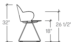
Ballad Plastic Outdoor Armchair Seat, Sled Base (TKDJWQ)
