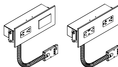
Module d'alimentation/communication horizontal – double (EPDHDFJ)
