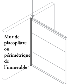
Raccord mural ou raccord mural réglable (FKW/FLKW)
