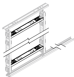
F K W Raccord mural Xpress
