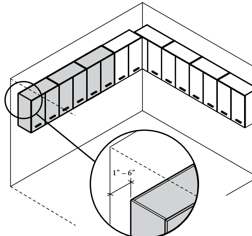
Step 4: Fill the other wall with cabinets. Leave a gap between 1" and 6" at the end as installer can cut to fit within wall conditions
