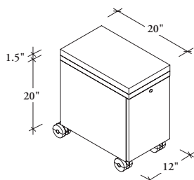
side drawer (S) 1 Lock
