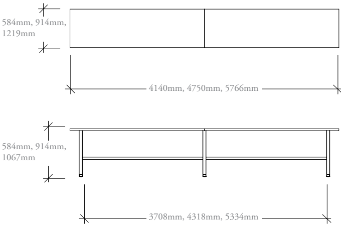
Ganged single top workshop tables
