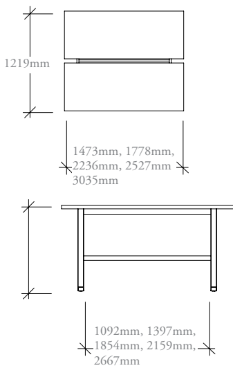
Split top workshop table
