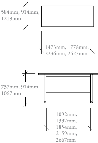
Single top workshop table
