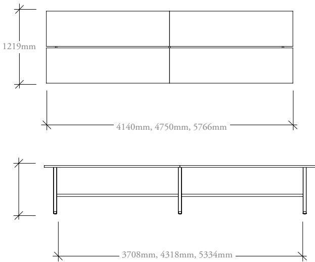
Ganged split top workshop tables
