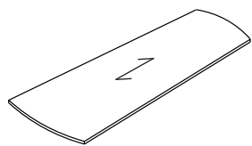
Wedge Shaped Conference Table Top with Bow Ends, Grain Runs Lengthwise
