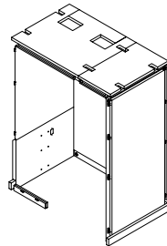
EFTWMA Tek Work Monoleg Worksurface Assembly
