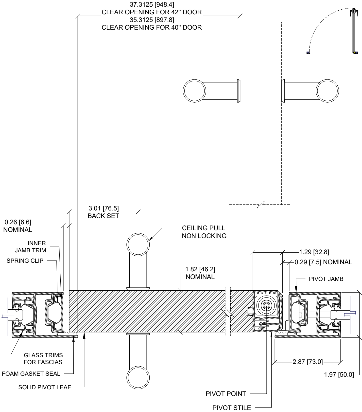
2/H SOLID PIVOT DOOR LEAF SINGLE B02 WITH JAMB AND CEILING PULL NON LOCKING
