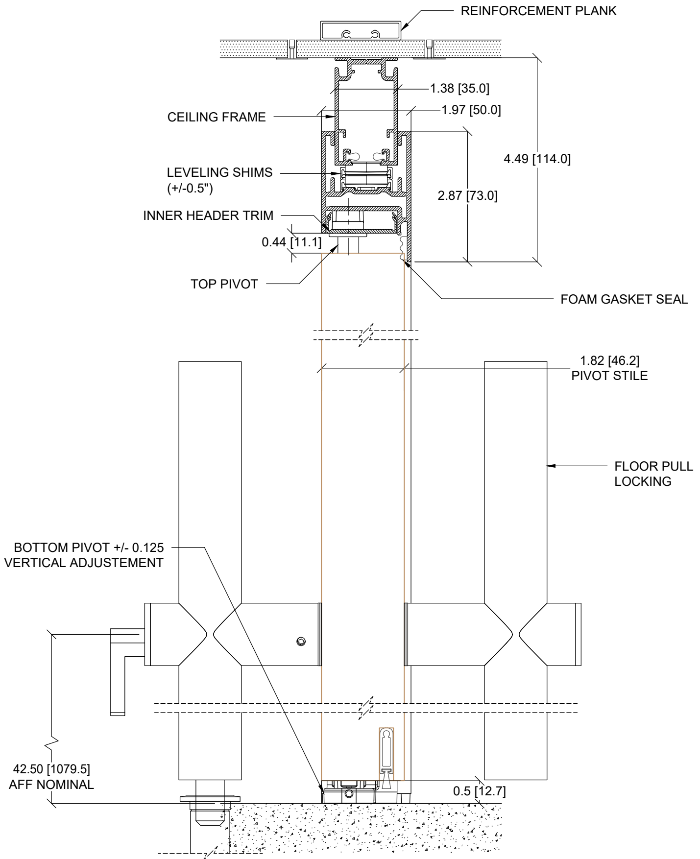
3/V B02 SOLID PIVOT DOOR LEAF SINGLE WITH JAMB AND FLOOR PULL LOCKING
