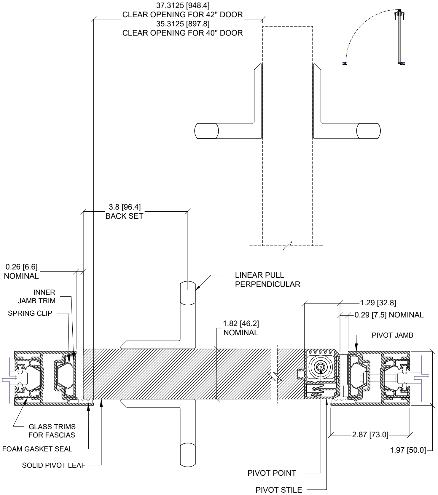
5/H SOLID PIVOT DOOR LEAF SINGLE B02 WITH JAMB AND LINEAR PULL PERPENDICULAR
