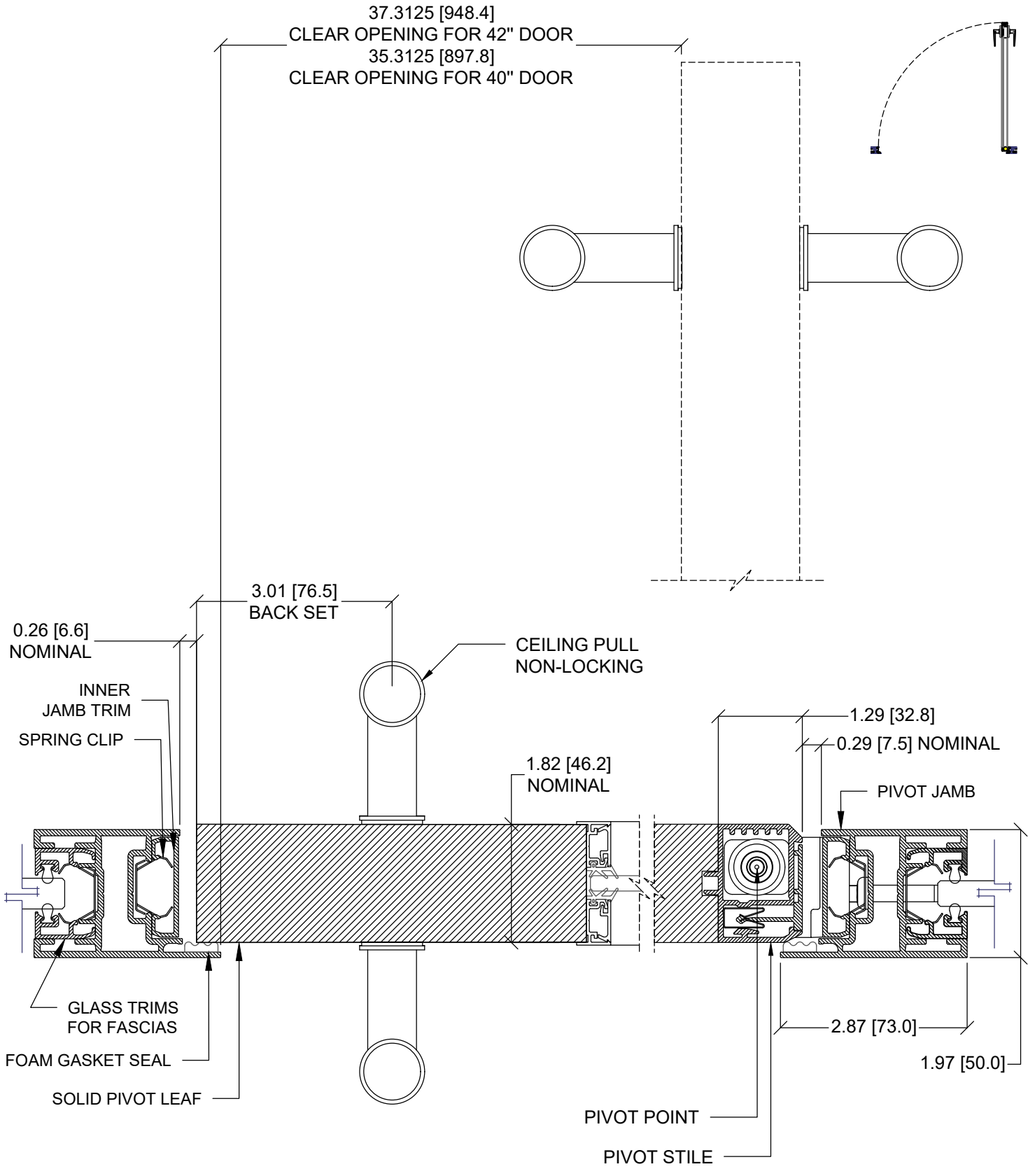
2/H SOLID PIVOT DOOR LEAF WITH GLASS INSERT SINGLE B04 WITH JAMB AND CEILING PULL
