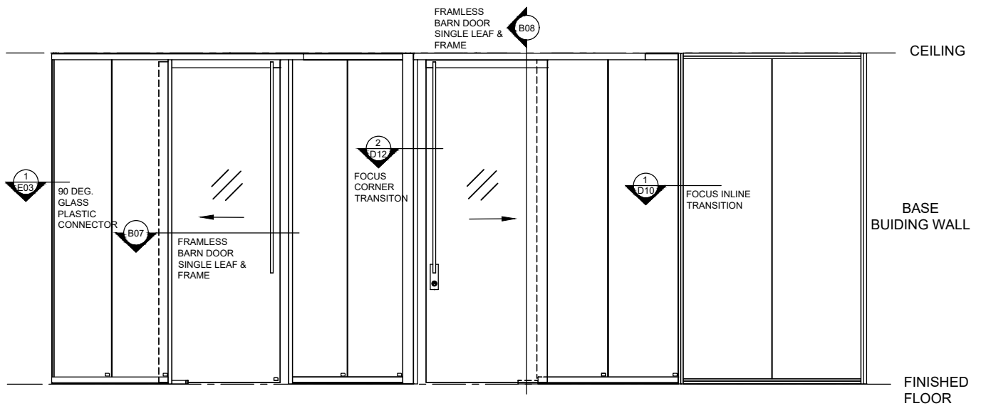
1 ELEVATION EL2
