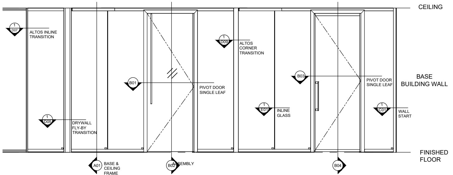
1 ELEVATION EL1
