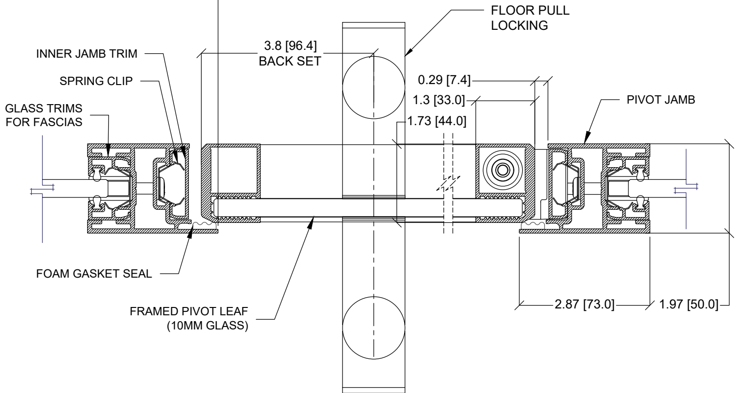
4/H B06 FRAMED 45MM SINGLE GLAZED PIVOT DOOR LEAF, SINGLE WITH JAMB AND FLOOR PULL NON-LOCKING
