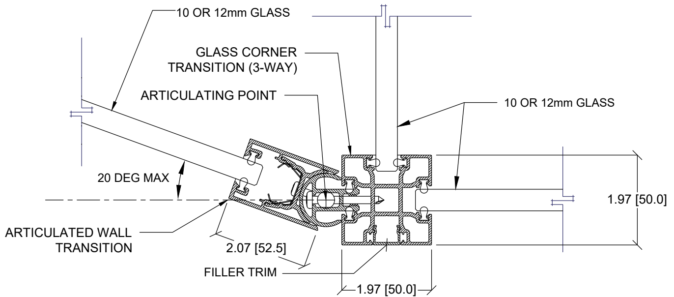
1 ARTICULATED TRANSITION D06 3-WAY GLASS CORNER
