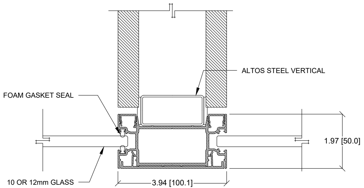
5 ALTOS TRANSITION D04 3-WAY GLASS TO GLASS
