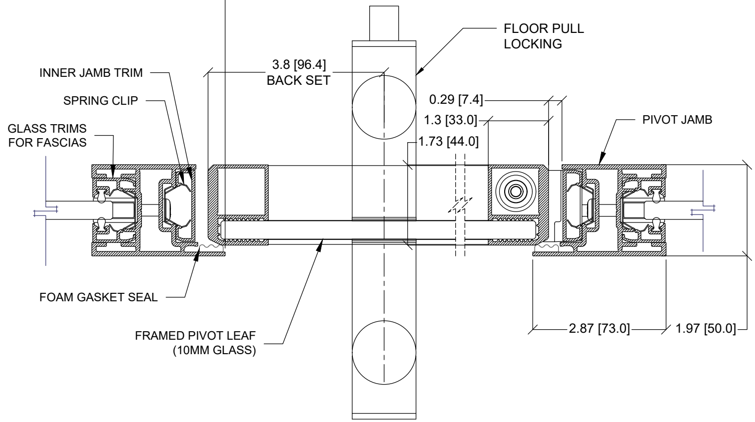
3/H B06 FRAMED 45MM SINGLE GLAZED PIVOT DOOR LEAF, SINGLE WITH JAMB AND FLOOR PULL LOCKING
