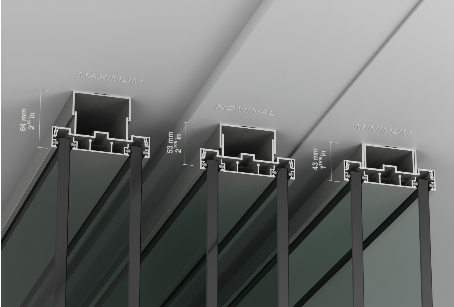
CEILING ADJUSTMENT
