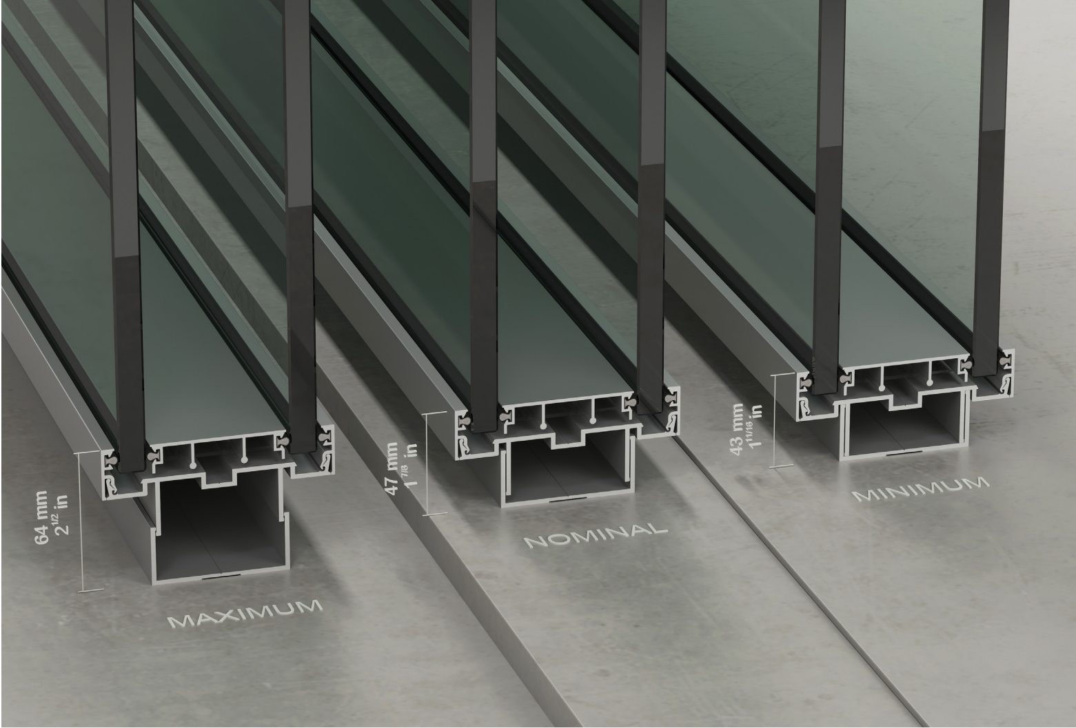
BASE ADJUSTMENT
